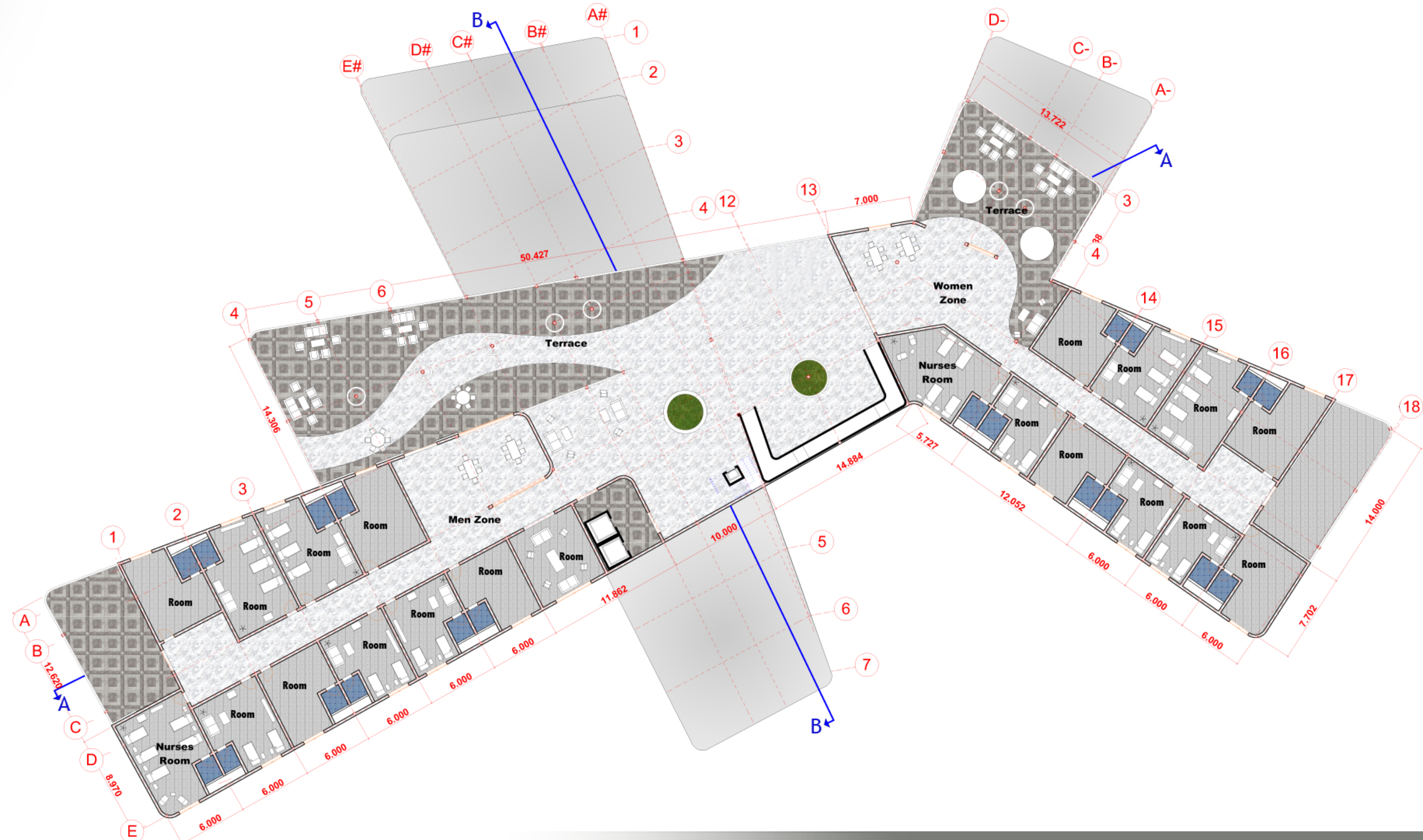
TYPECAL FLOOR PLAN SCALE 1:200
