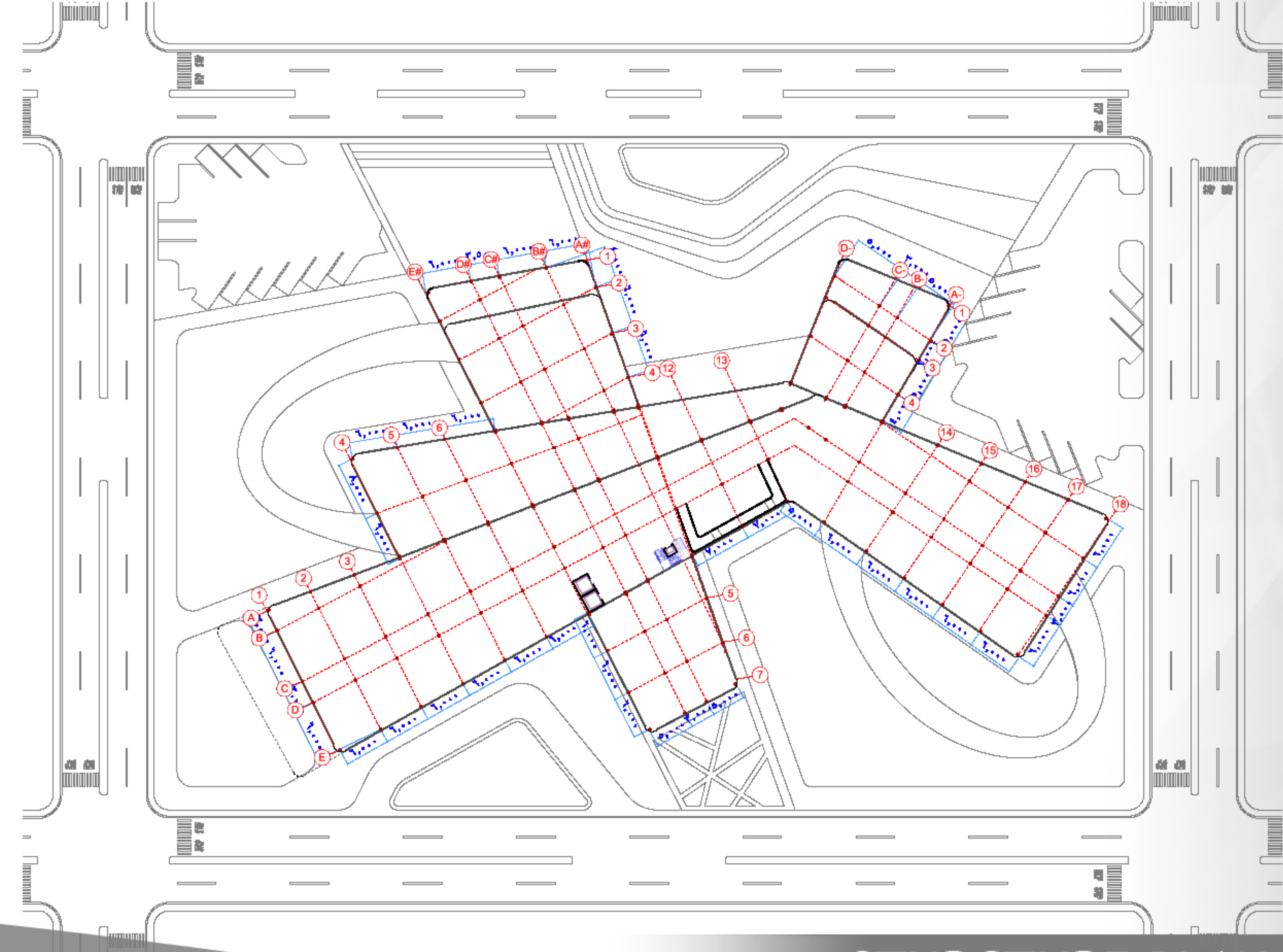
STURCTURE PLAN
