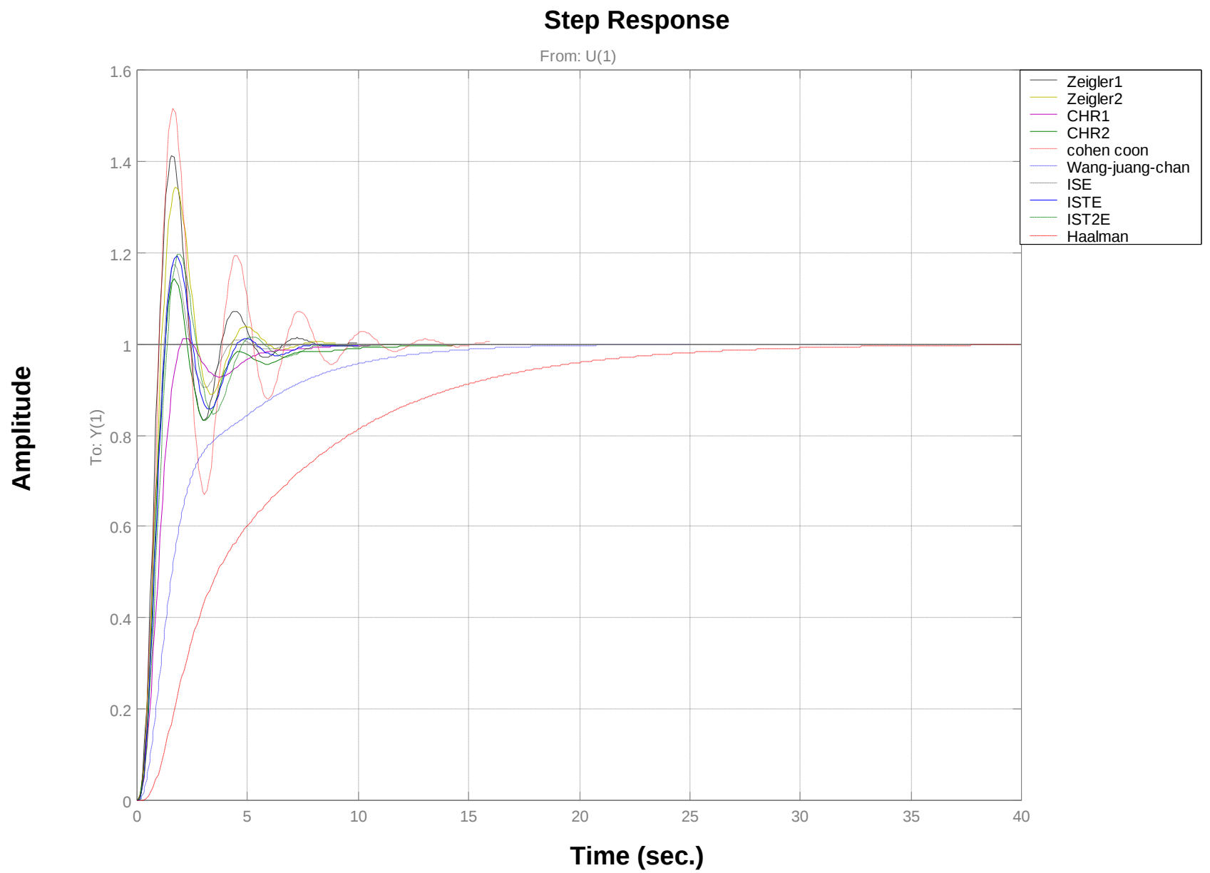
Fig. (4.14): Close-loop step responses from all method
