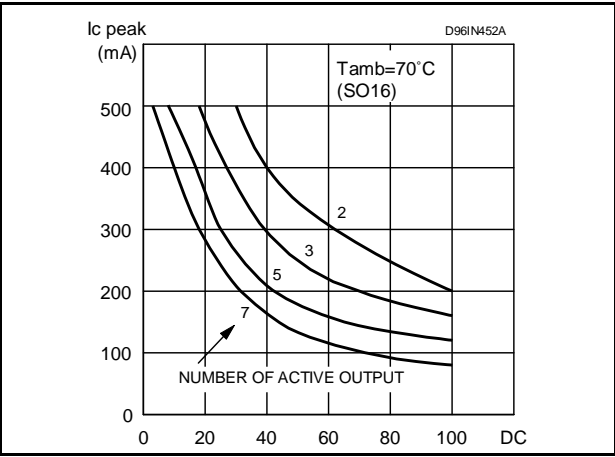
Figure 13. Peak collector current vs duty cycle Figure 14. Peak collector current vs duty cycle
