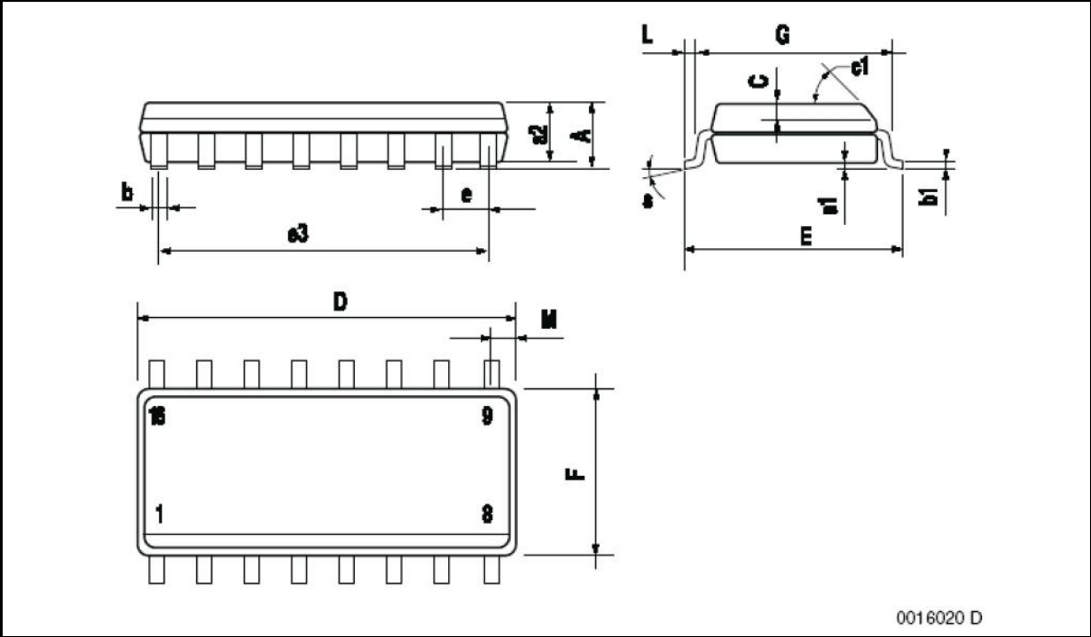
Figure 15. Package dimensions
