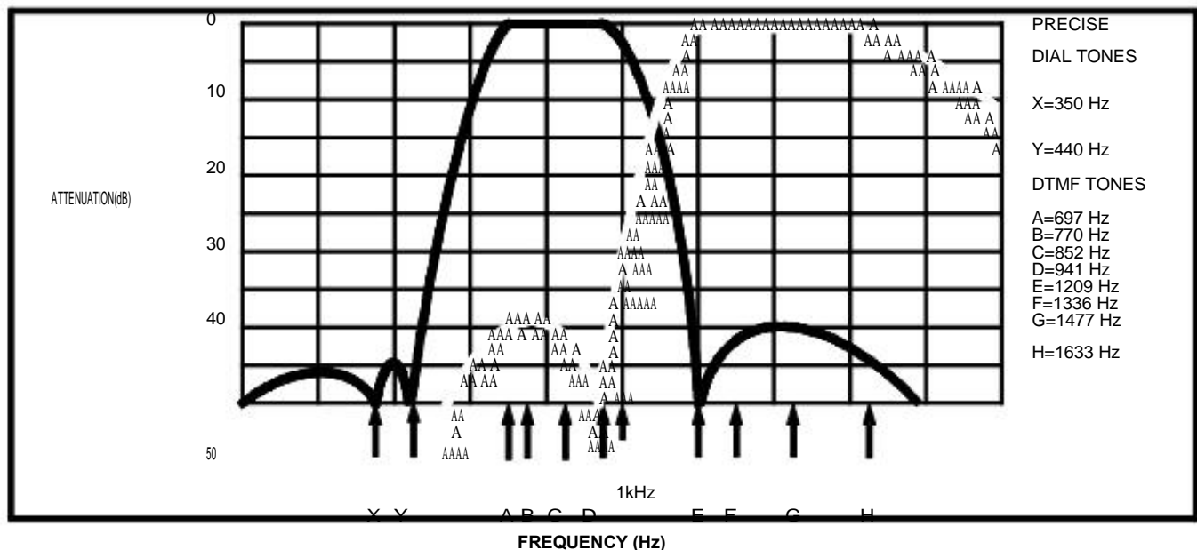
Figure 3 - Filter Response
