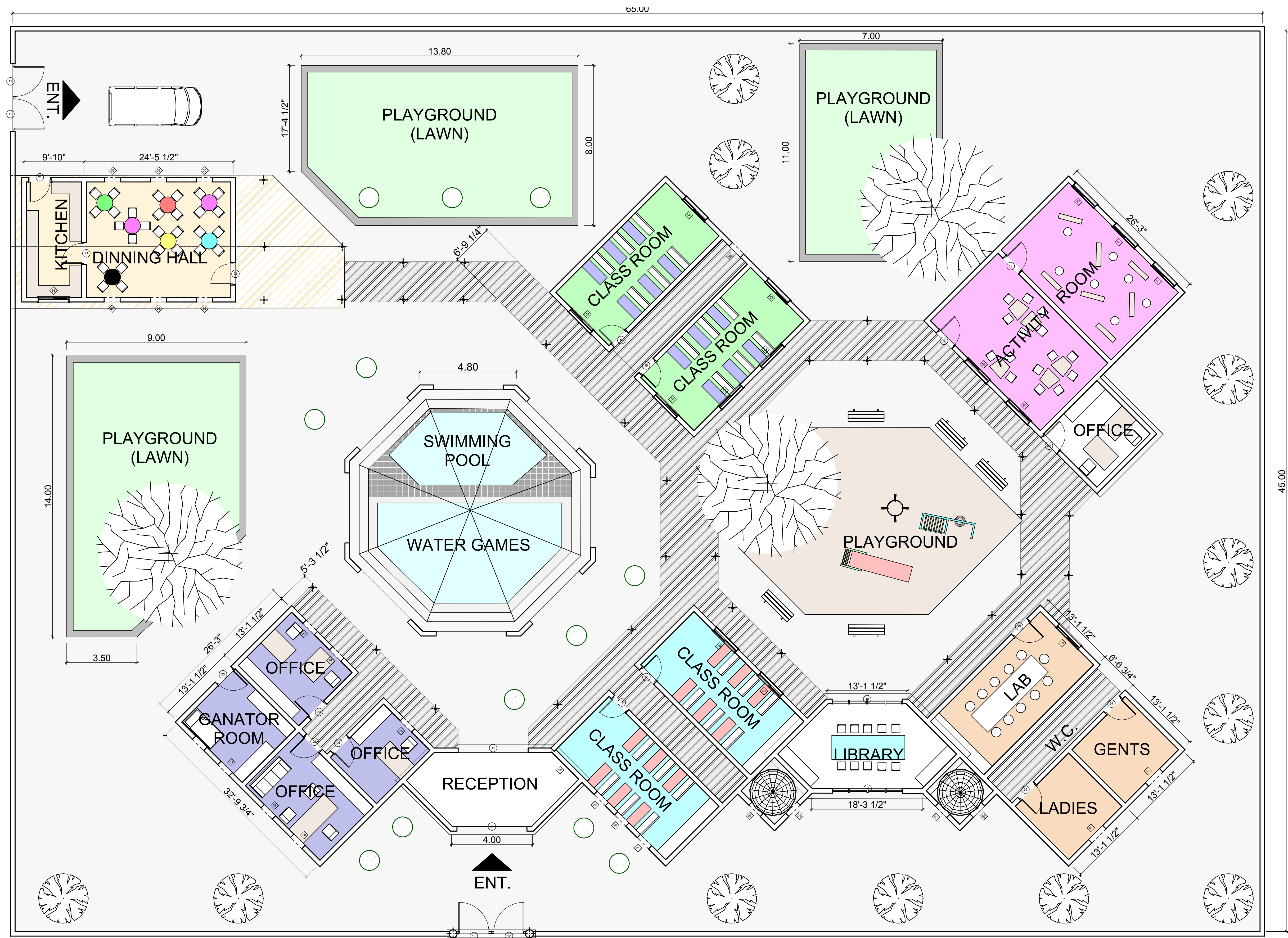
1 GROUND FLOOR PLAN
