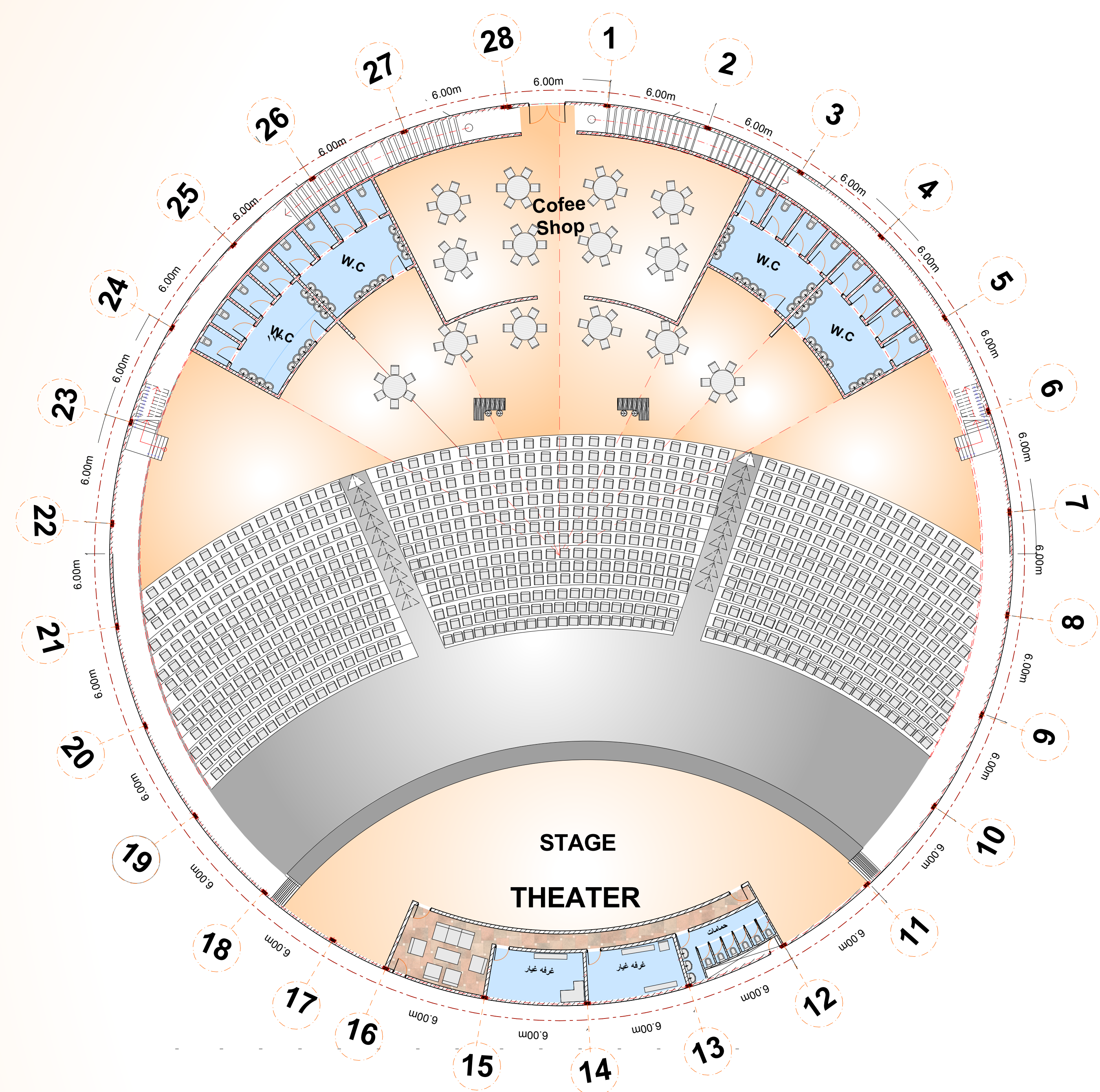
A GROUND FLOOR PLAN SCALE 1:200
