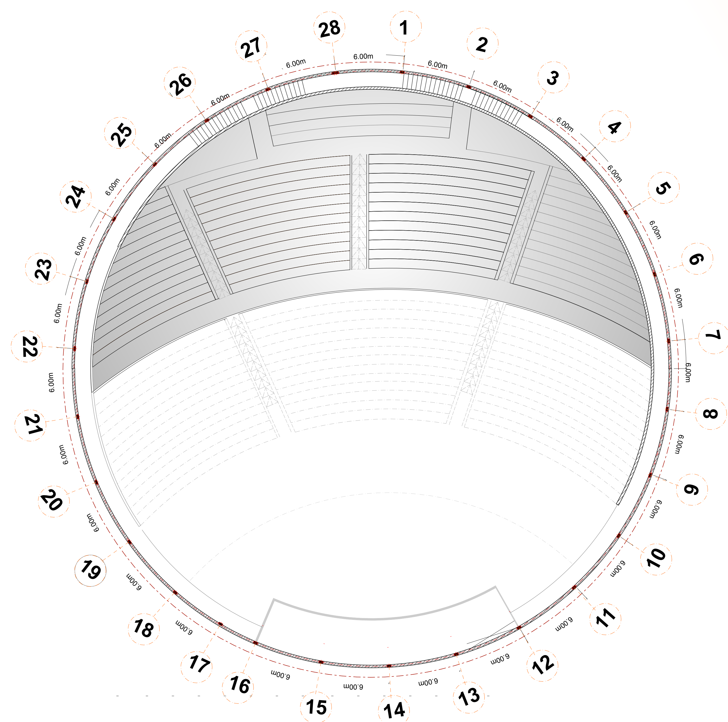
SECOND FLOOR PLAN SCALE
