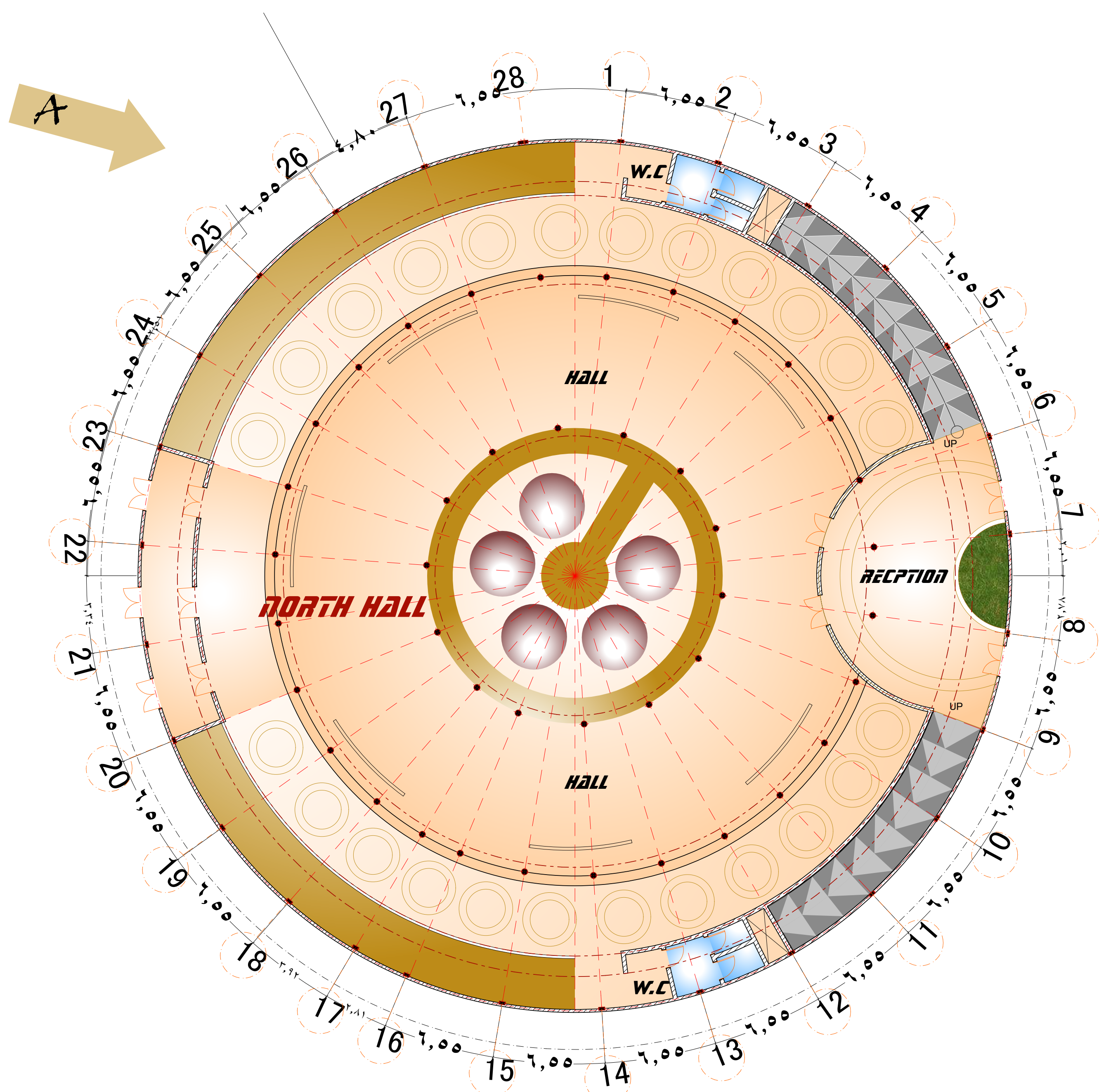
A GROUND FLOOR PLAN NORTH HALL
