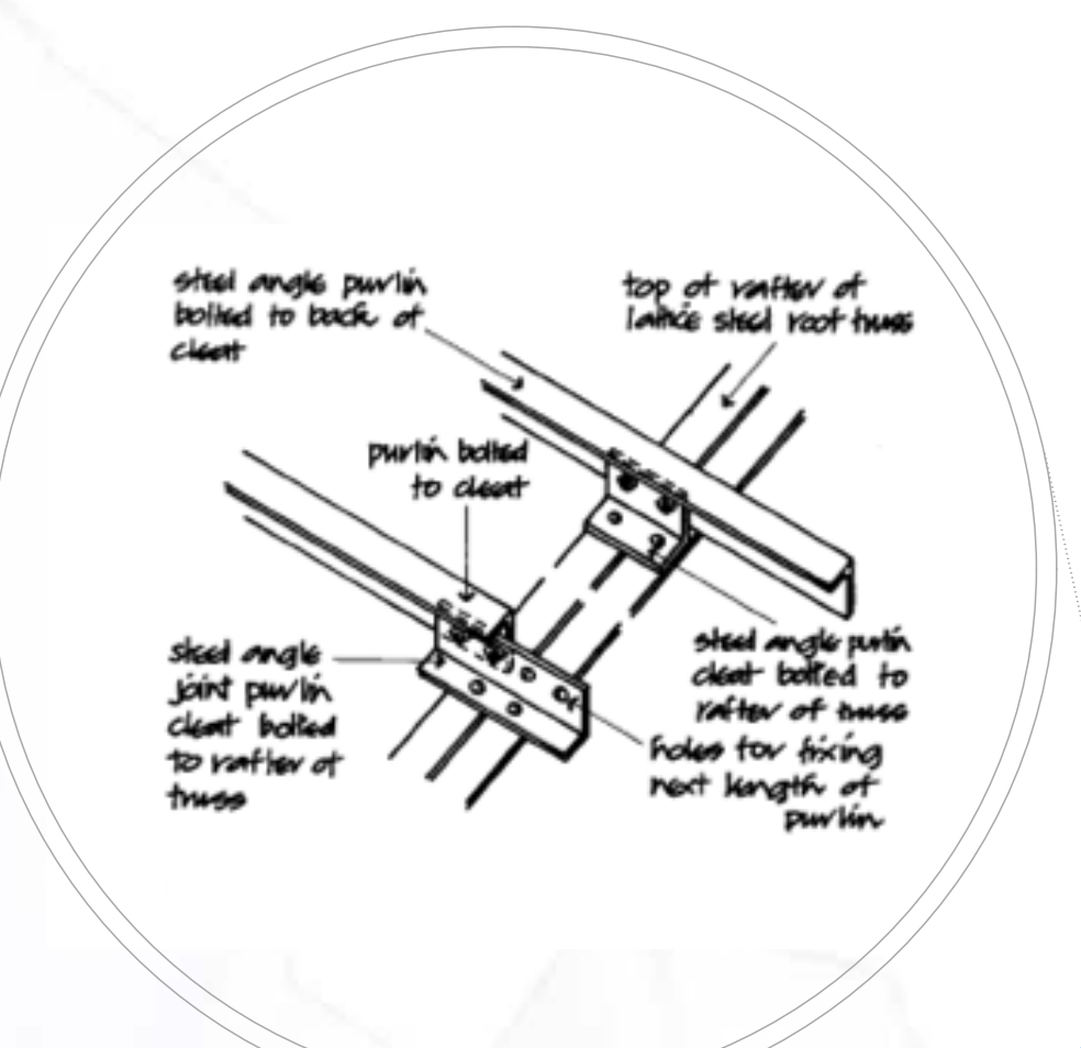
PURLIN CONNECTION WITH GIRDER BEAM
