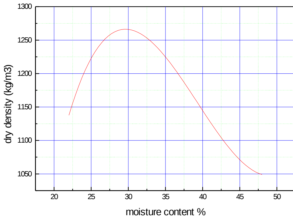
Fig(4.6): Compaction Test (FAO Project)
