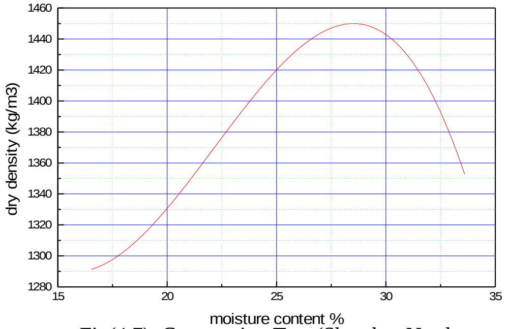
Fig(4.7): Compaction Test (Shambat-North Khartoum)
