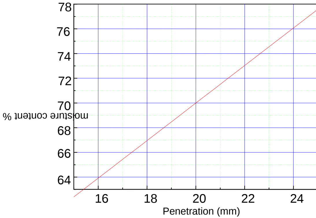
Fig(4.5): Atterberg Limits (Almenshia-Khartoum )
