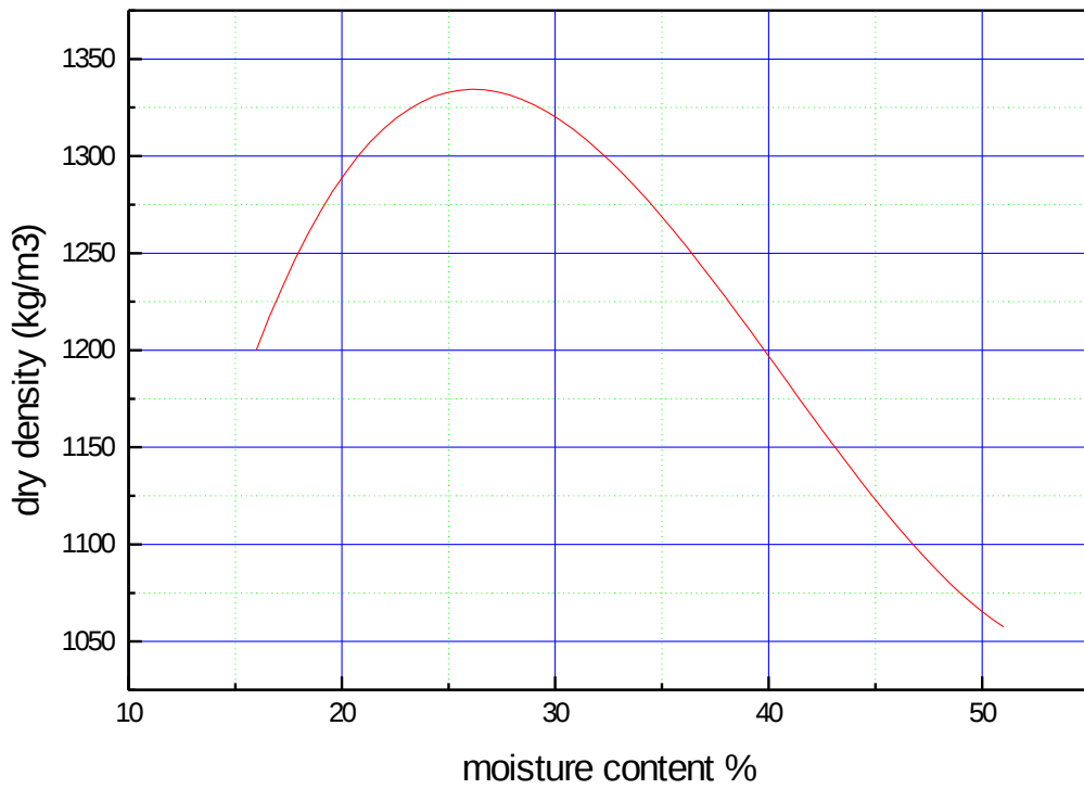
Fig(4.8): Compaction Test (Almenshia-Khartoum)
