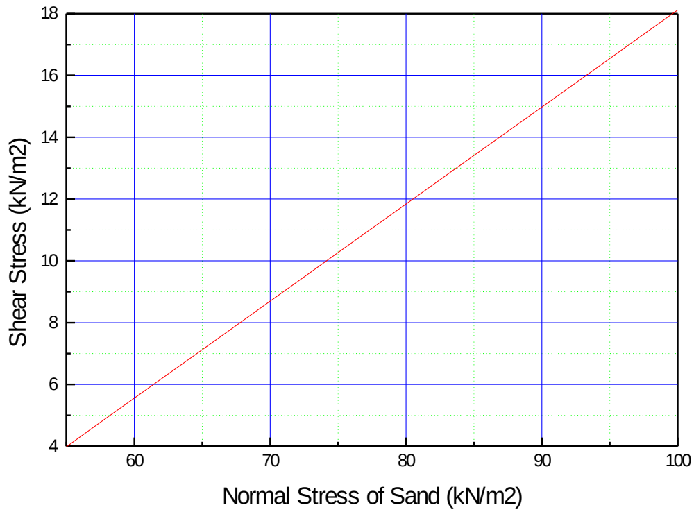
Fig(4.2): Direct Shear Box Test of Sand
