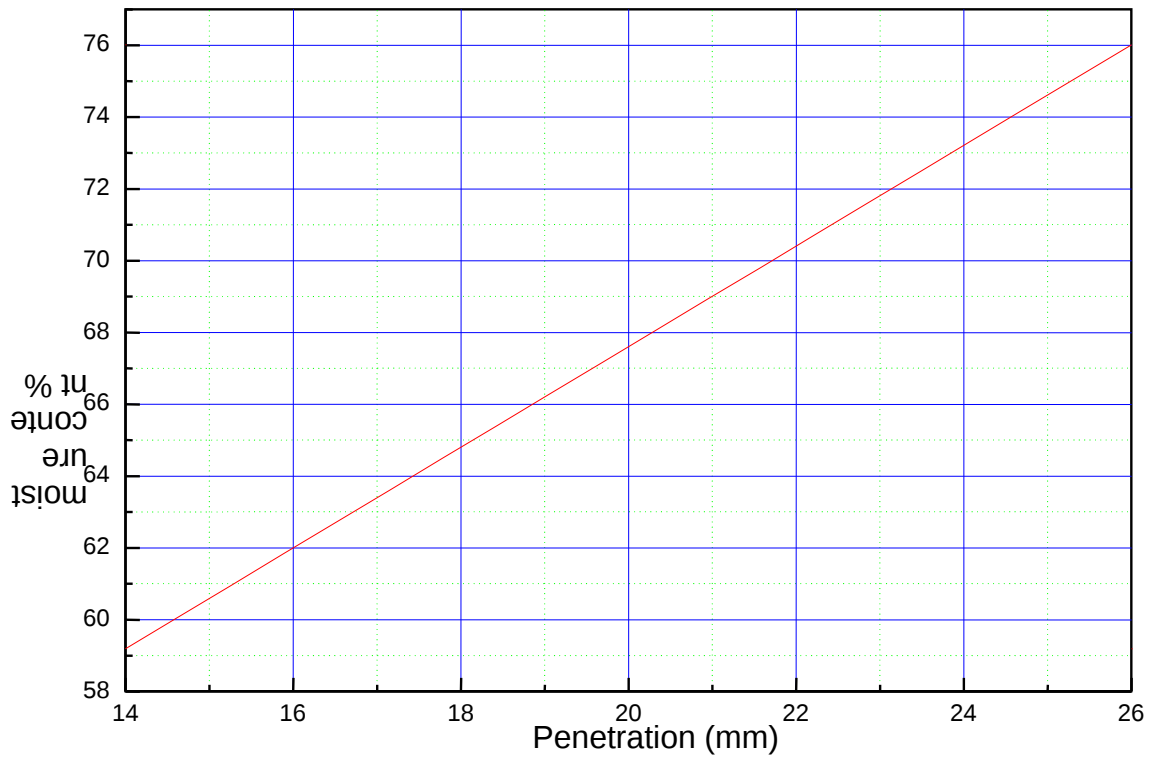
Fig(4.4): Pentrometer test. Atterberg Limits (Shambat- North Kkartoum)
