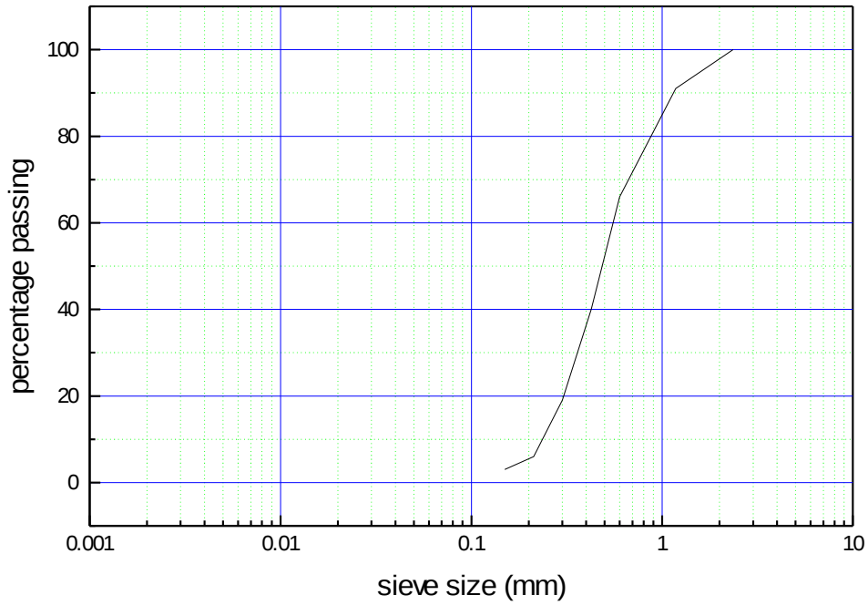
Fig(4.1): Particle Size Distribution of Sand
