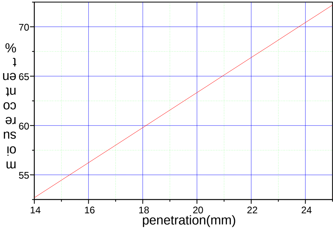
Fig(4.3): Pentrometer test. Atterberg Limits (FAO- Project)
