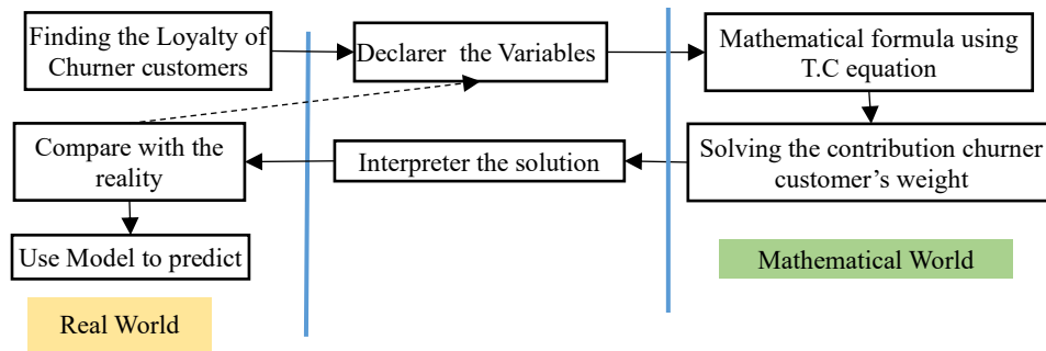
Figure 2. Mathematical Model
