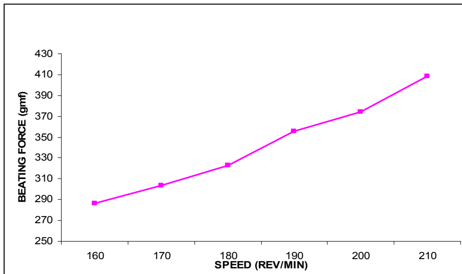
Figure 3: The Beating Force as Function of Loom Speeds
