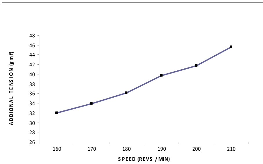
Figure 4: The Additional Yarn Tension ( \Delta T_y ) Caused By the Beating Action at Different Loom Speeds
