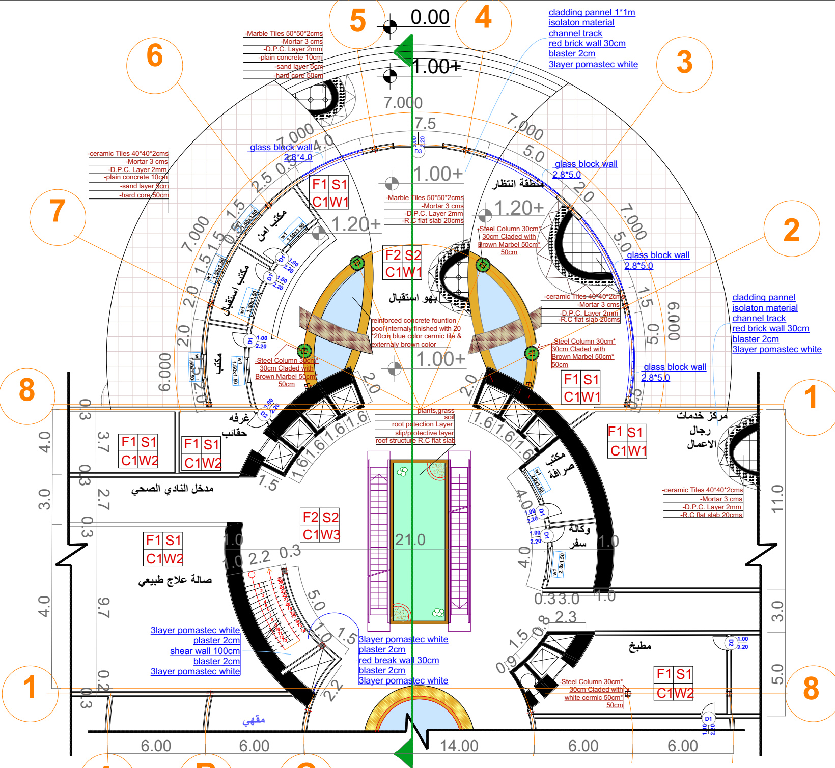
foyer part plan-scale 1:50
