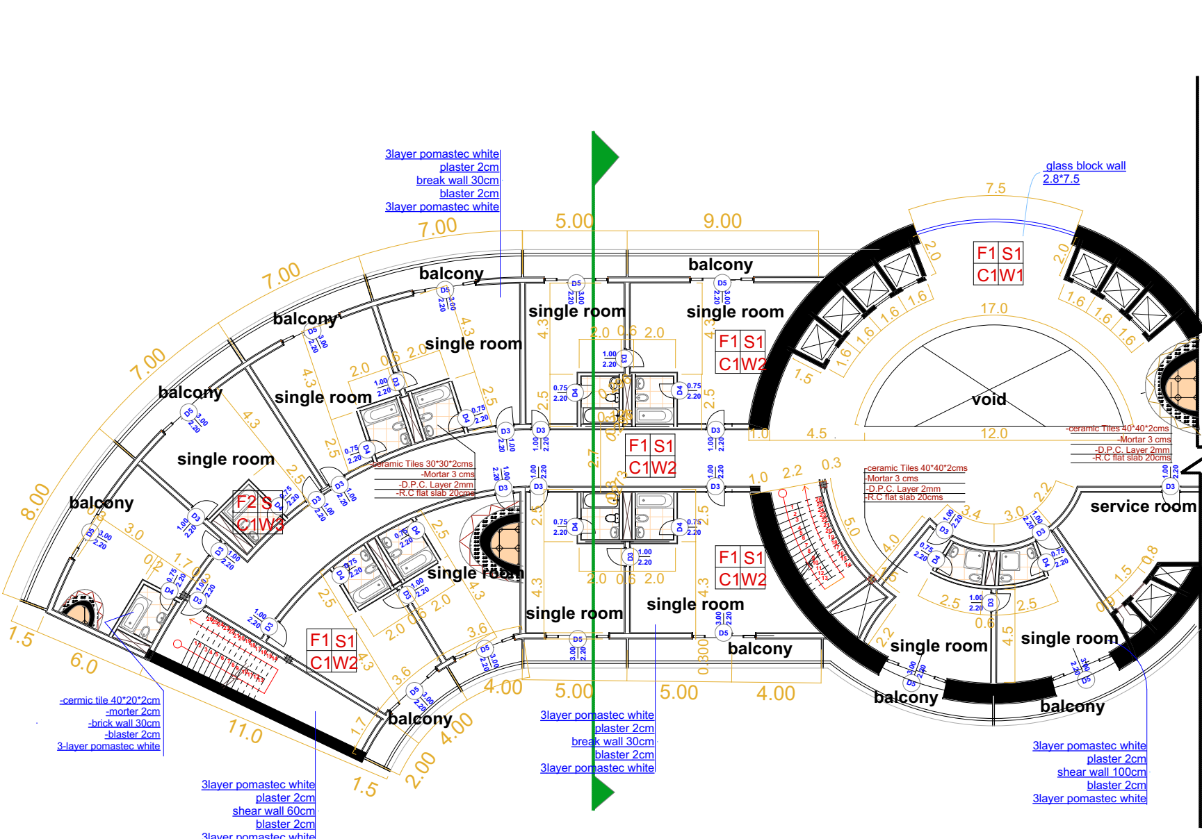
rooms part plan-scale 1:50
